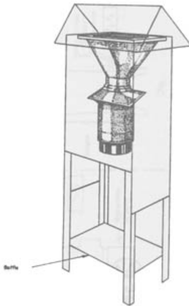
Figure 1. High-volume sampler in shelter.
